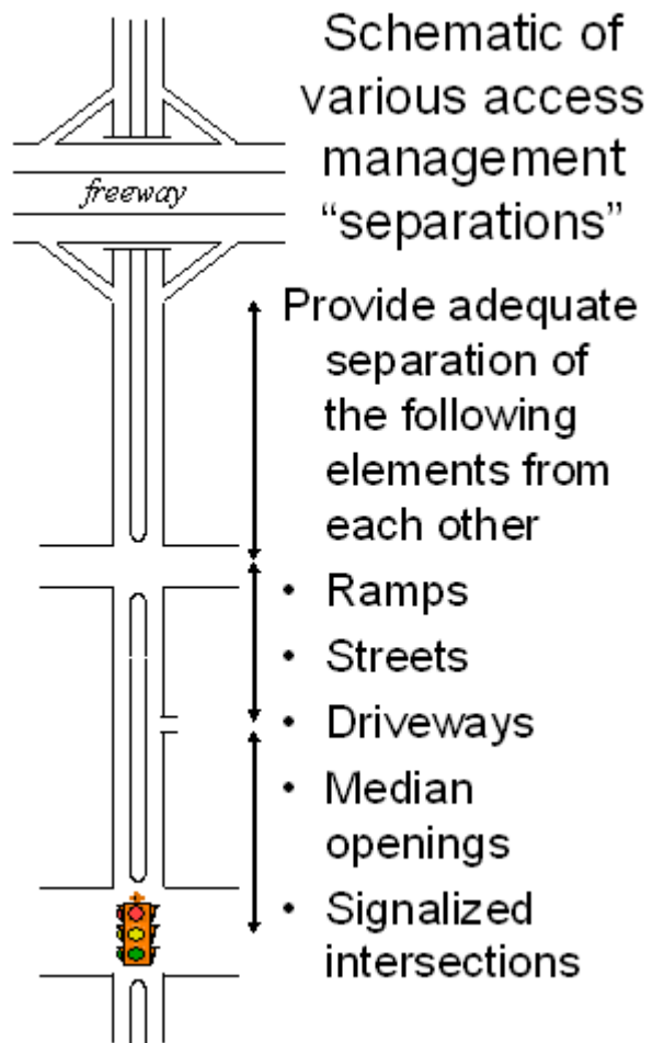
EXHIBIT 3-7 Some locations at which to manage access
