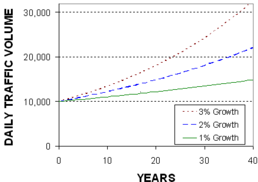
EXHIBIT 5-2 Effect of traffic growth on volume thresholds
