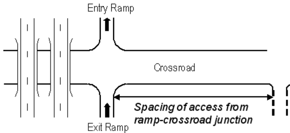
EXHIBIT 3-19 Access spacing at ramp-crossroad junctions
