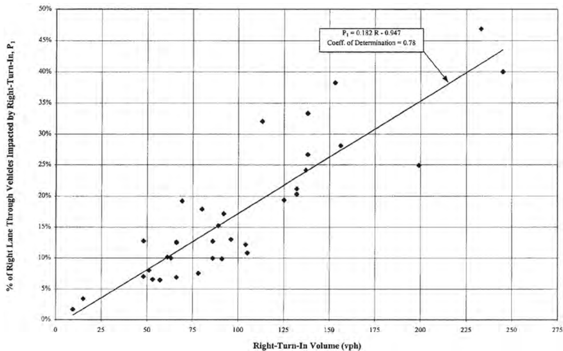
EXHIBIT 2-17 Percentage of through vehicles in right lane affected by right-turn vehicles
