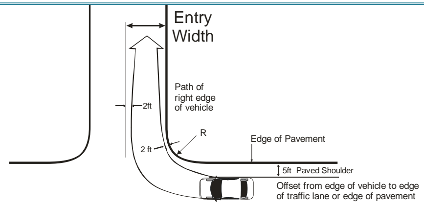
Exhibit 14 Important Measures that Determine the Entry Operations of a Driveway
