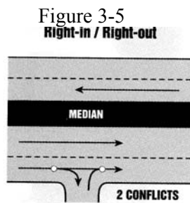
Figure 3-2, 3-4 and 3-5 Source: Michigan Department of Transportation, Improving Driveways and Access Management in Michigan , 1996, p. 4. Figure 3-3 Source: National Highway Institute, Course 15255, FHWA, 1998, p. 4-8.
