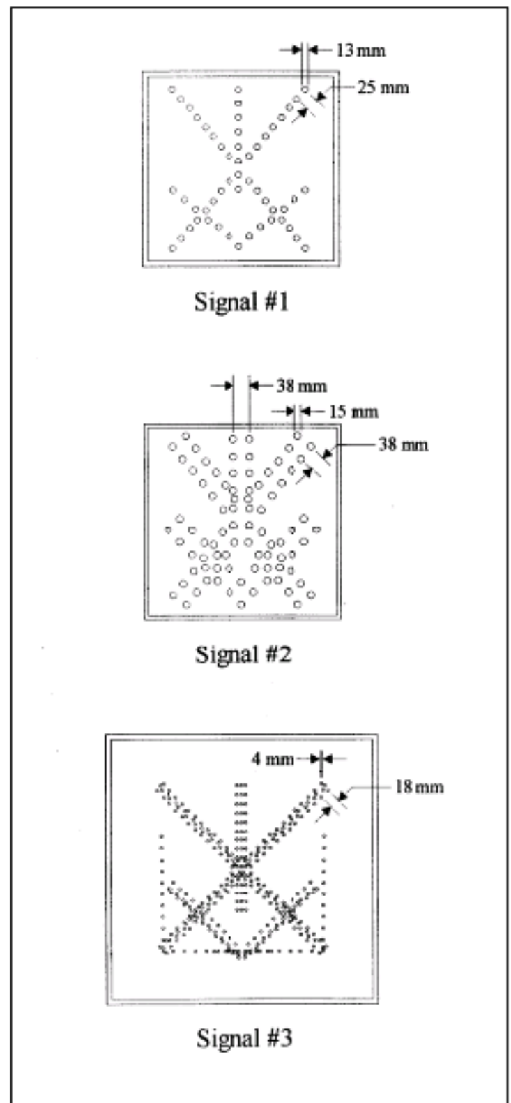
Figure 21. Pixel layout of LSC heads employed in research conducted by Ullman et al., 1996.
