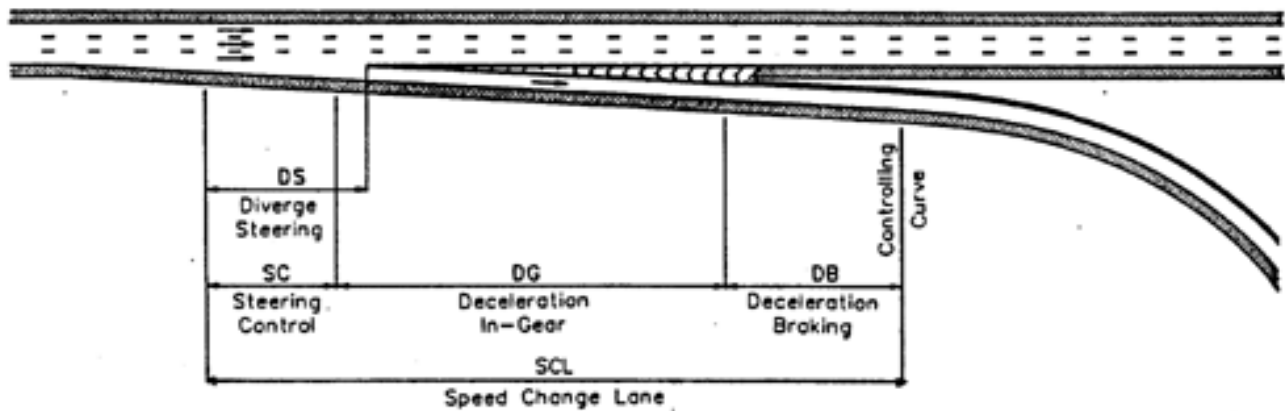
Figure 20. The exit process and components of the exit model developed in NCHRP 3-35.
