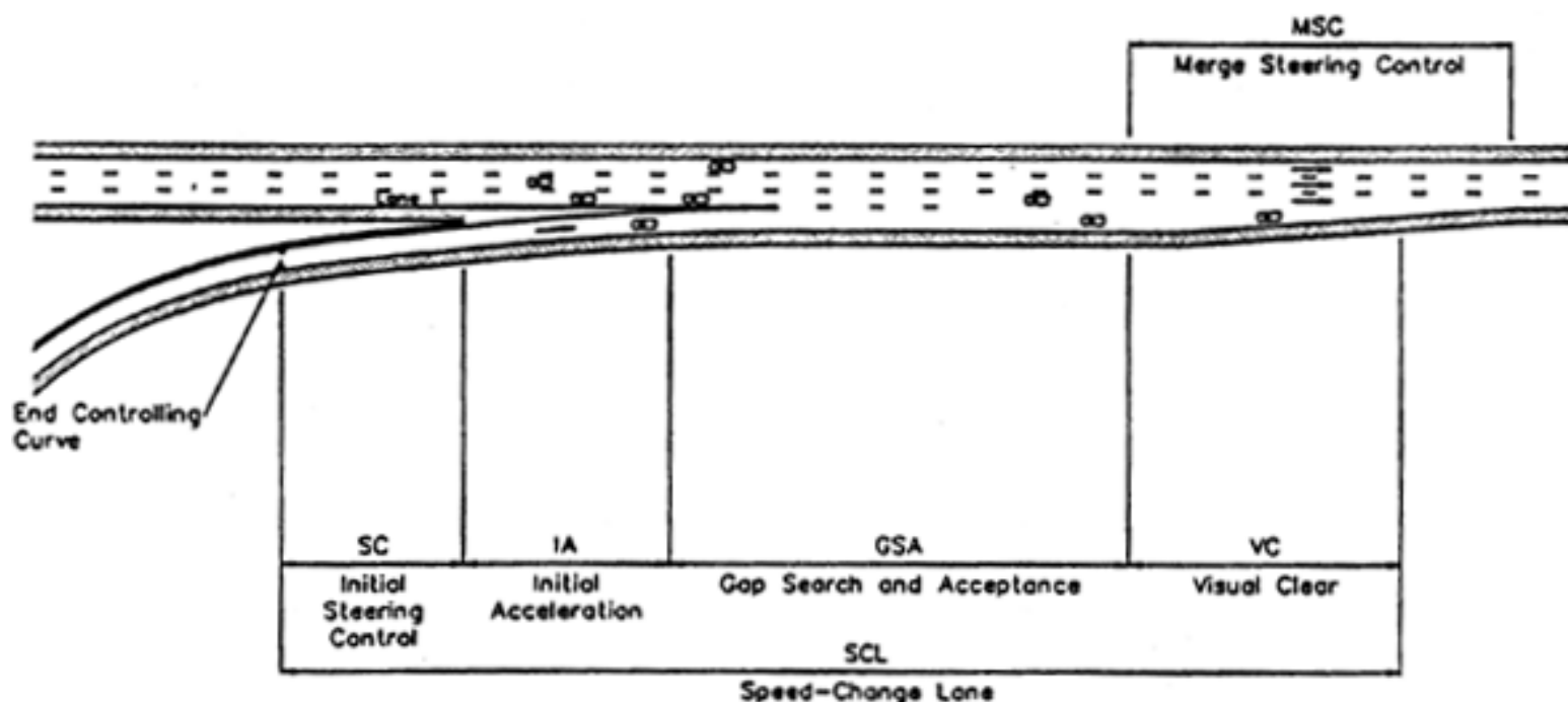
Figure 19. The entry process and components of the entry model developed in NCHRP 3-35.
