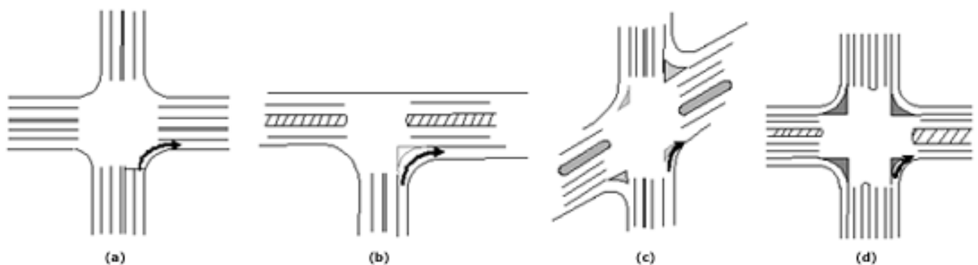
Figure 2. Intersection geometries examined in the Staplin et al.(1997) field study of right-turn channelization.
