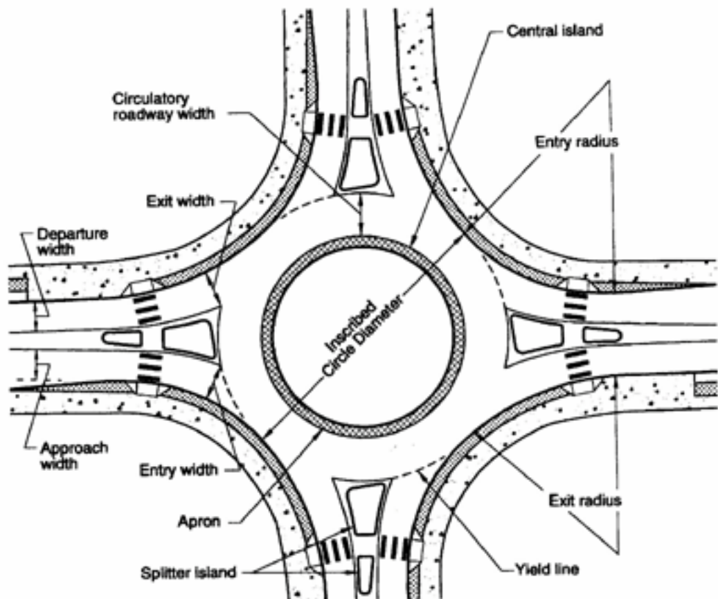
Basic geometric elements of a roundabout. Source: Roundabouts: An Informational Guide (FHWA, 2000)
