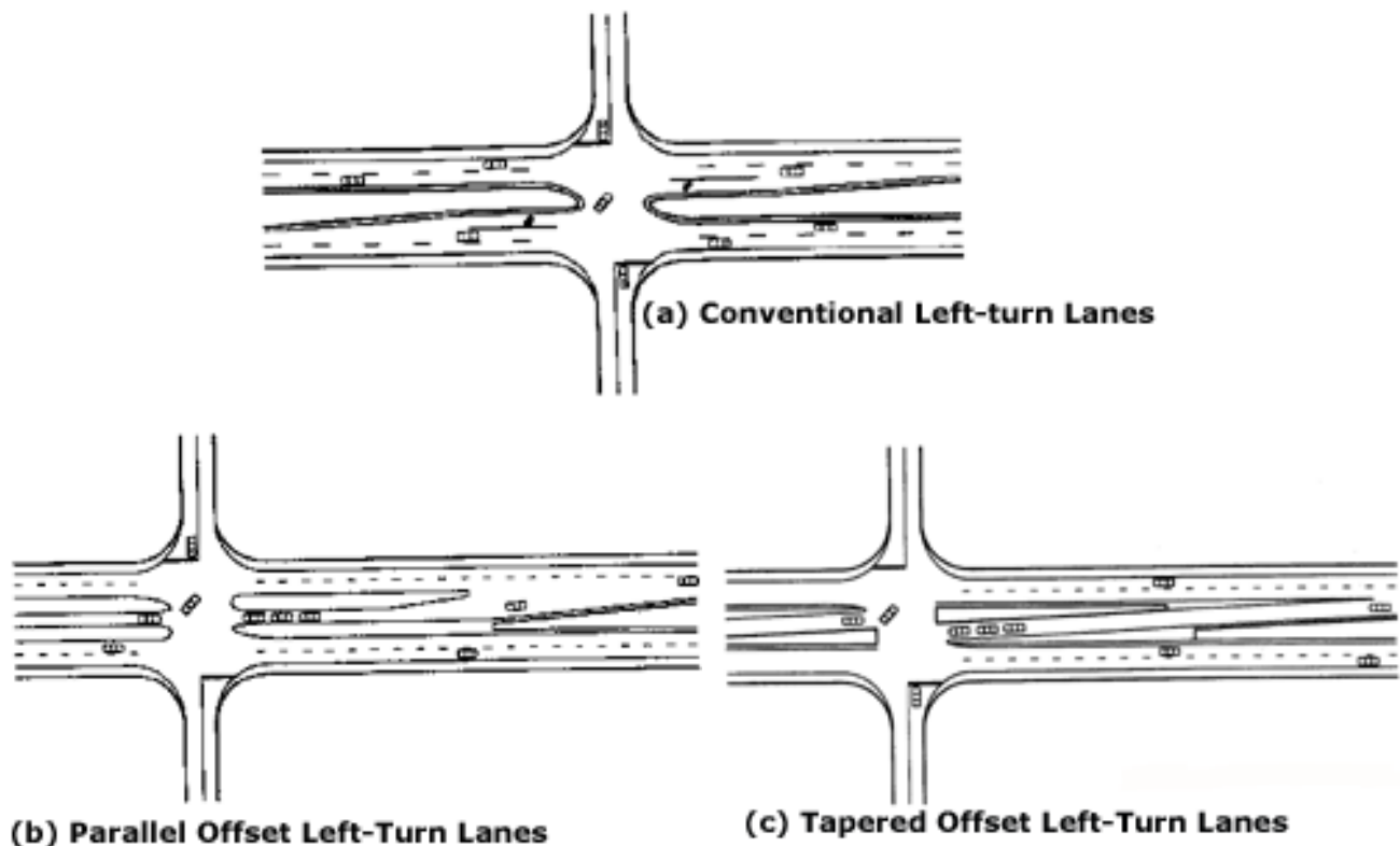
Figure 7. Alternative Left-turn treatments for rural and suburban divided highways.
