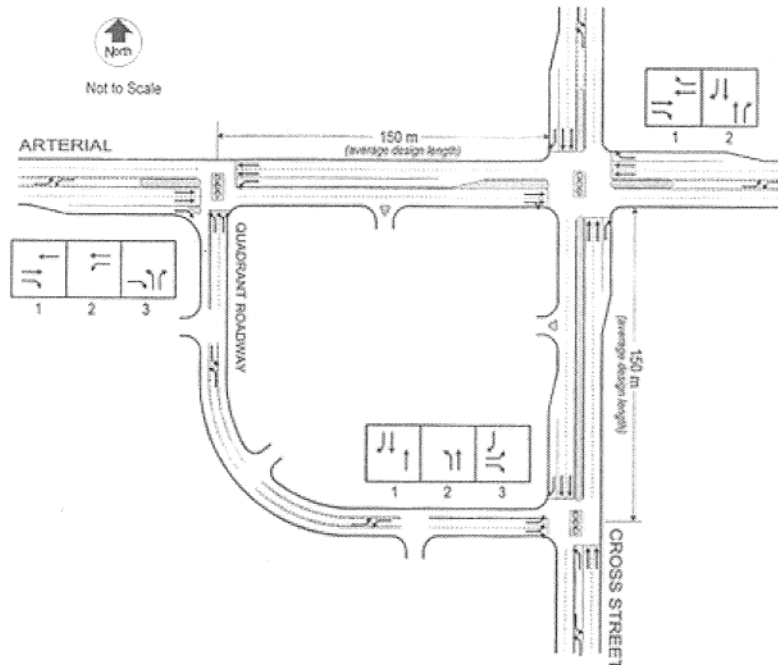
FIGURE 18 QRI design (176).
