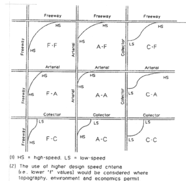
FIGURE 41 Minimum design speed criteria for ramp terminals (258).
